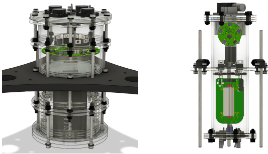
Figure 5: 3D models of Explorator chipper (left) and Explorator winder (right).
