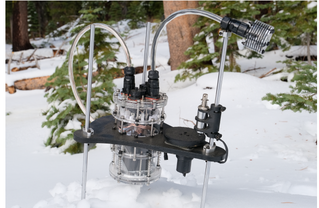
Figure 7: Explorator chipper .
